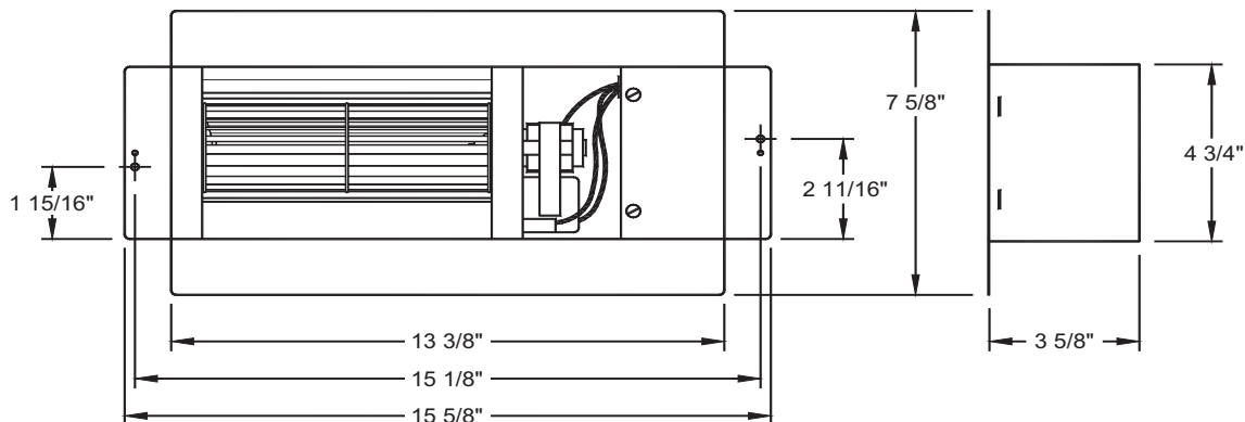
Front View
