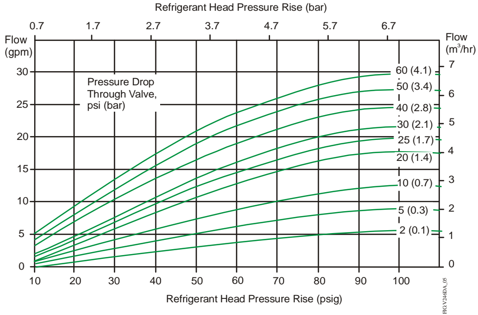
1/2 in. Direct Acting Valve Flowchart
