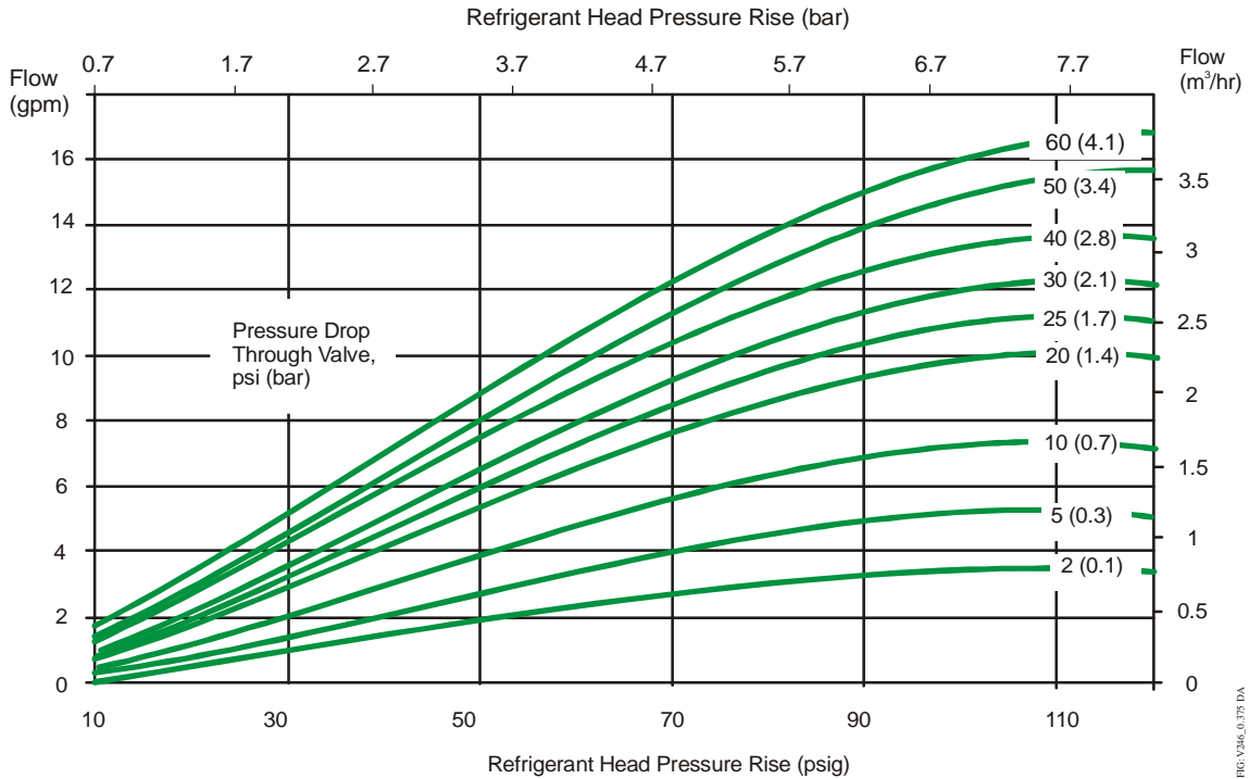
3/8 in. Direct Acting Valve Flowchart
