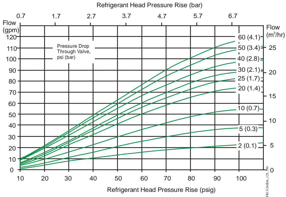
1-1/4 in. Direct Acting Valve Flowchart
