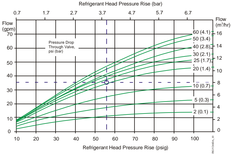
1 in. Direct Acting Valve Flowchart
