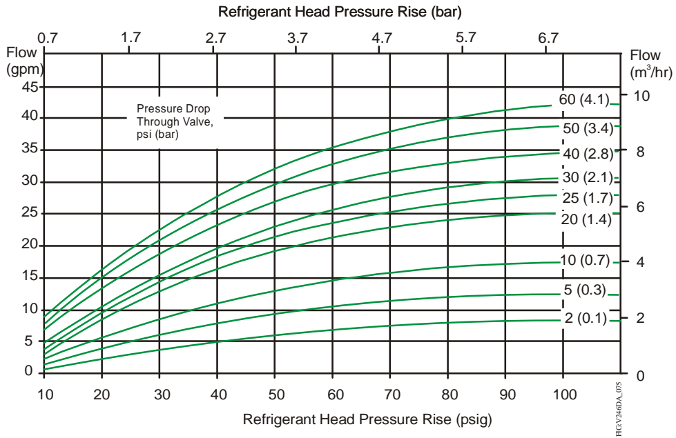
3/4 in. Direct Acting Valve Flowchart
