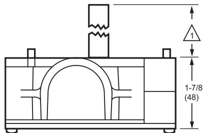
Fig. 1. Q5020 Dimensions in in. (mm).
