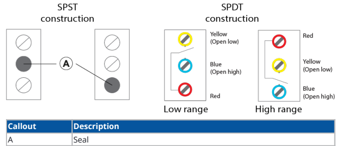
Figure 2: Terminal constructions
